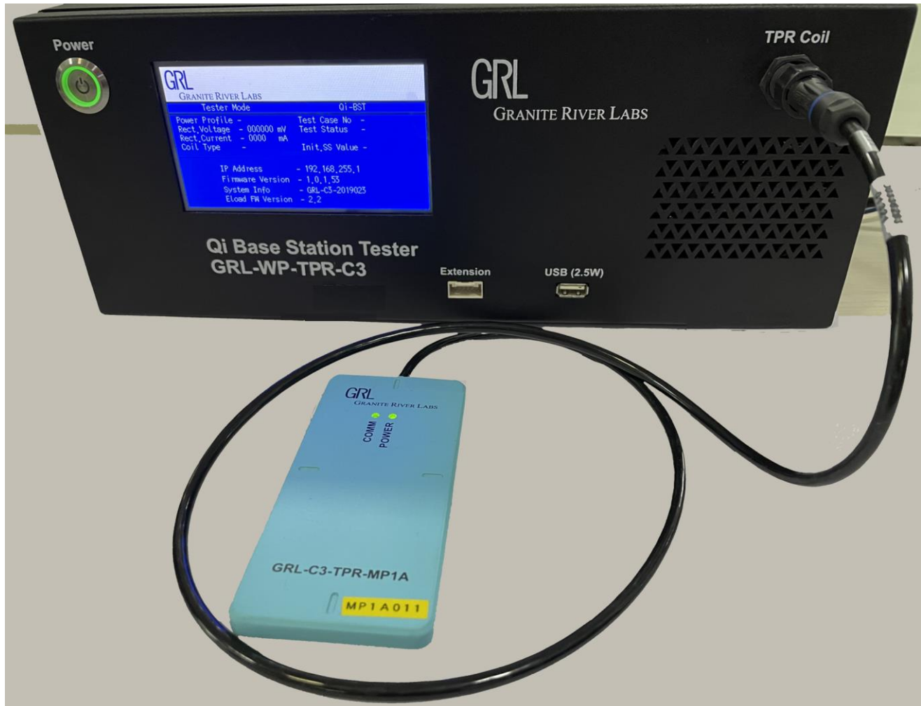
FIGURE 6.10: TPR COIL TO GRL-C3 CONNECTION
