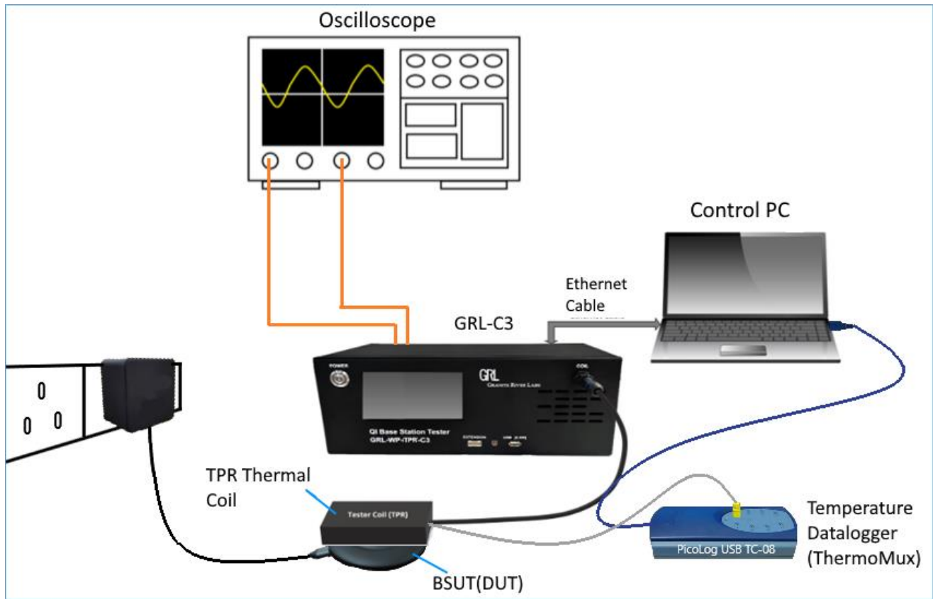
FIGURE 8.41: THERMOMUX CONNECTION SETUP DIAGRAM
