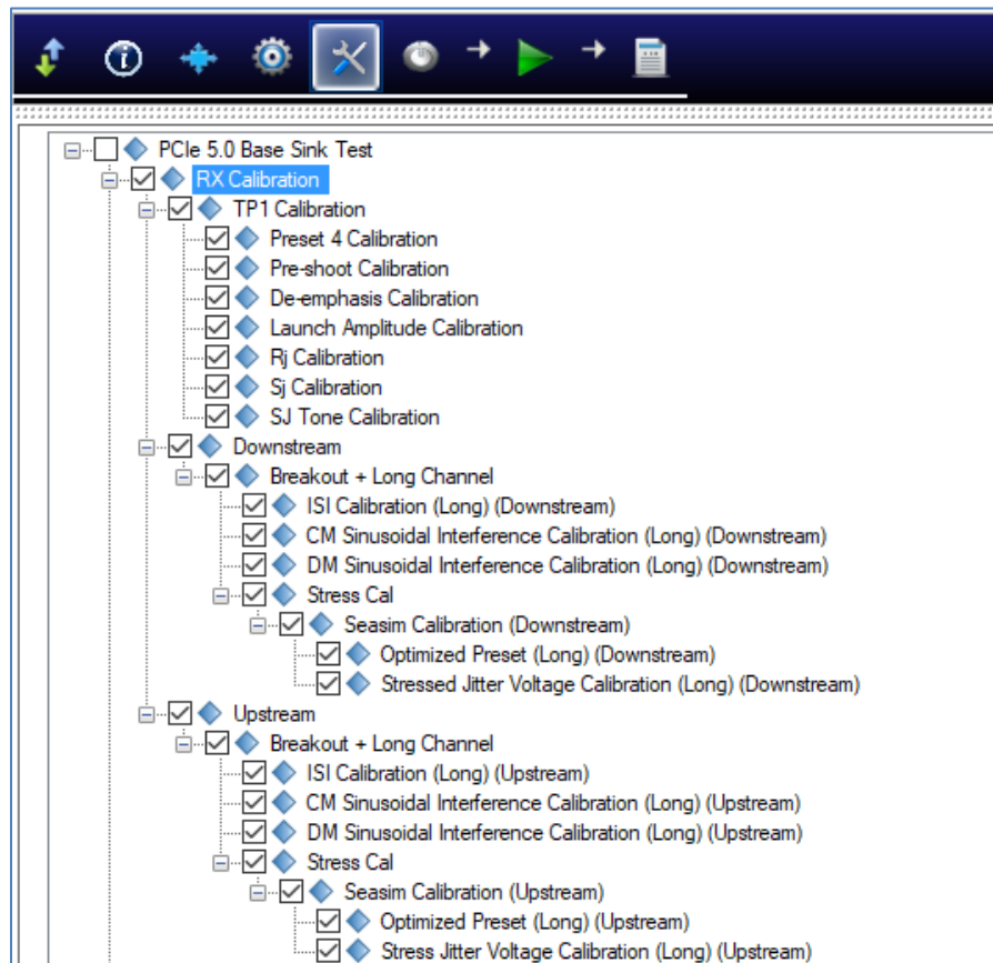
FIGURE 23. CALIBRATION SELECTION
