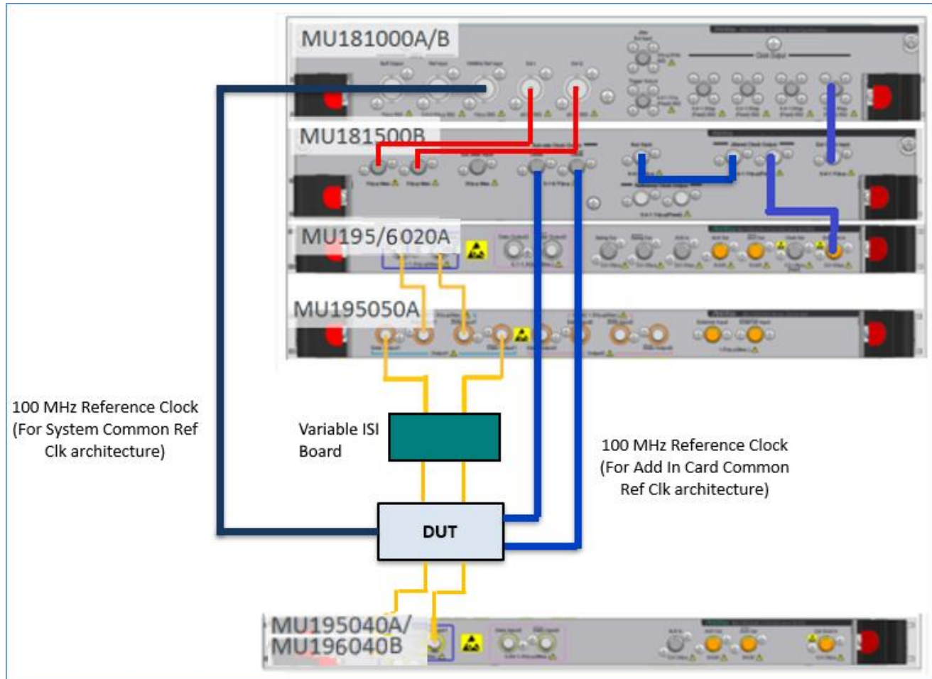
FIGURE 31. TYPICAL RECEIVER DUT TEST SETUP
