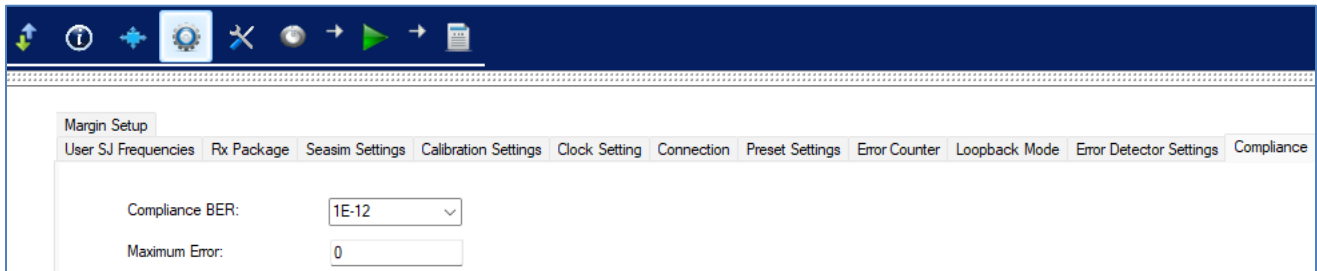
FIGURE 18. COMPLIANCE BER AND MAXIMUM ERRORS SETUP
