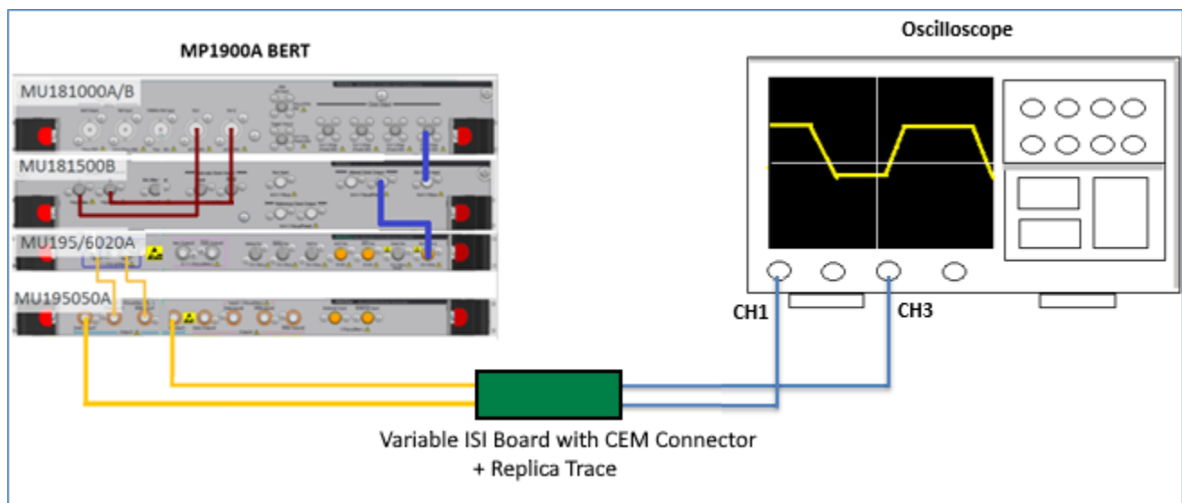
FIGURE 27. TYPICAL SETUP FOR TP2 CALIBRATION
