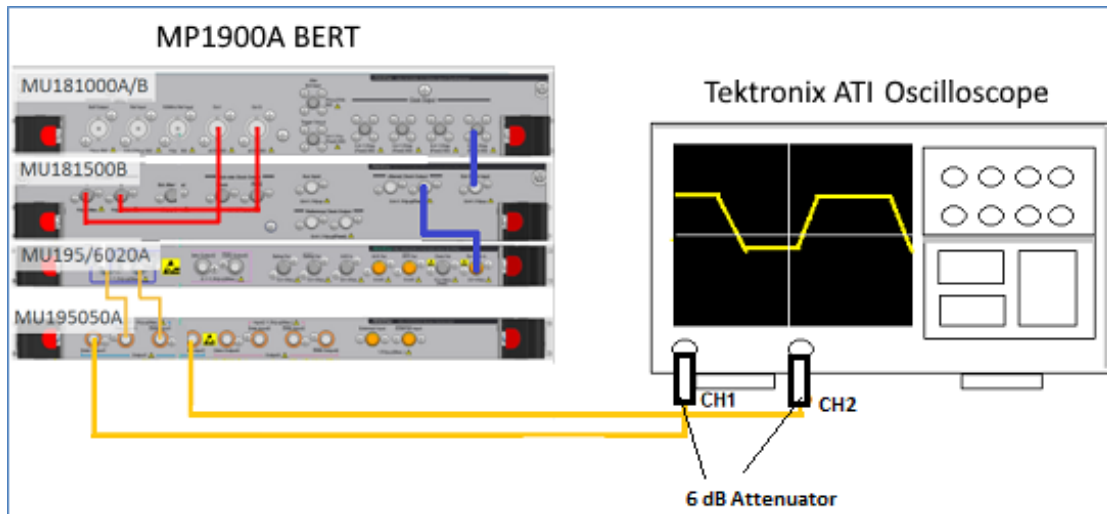
FIGURE 22. RECOMMENDED SETUP FOR TP1 CALIBRATION USING TEKTRONIX ATI SCOPE
