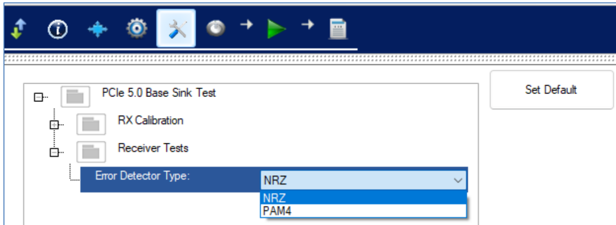
FIGURE 34. RECEIVER TEST PARAMETERS CONFIGURATION PAGE
