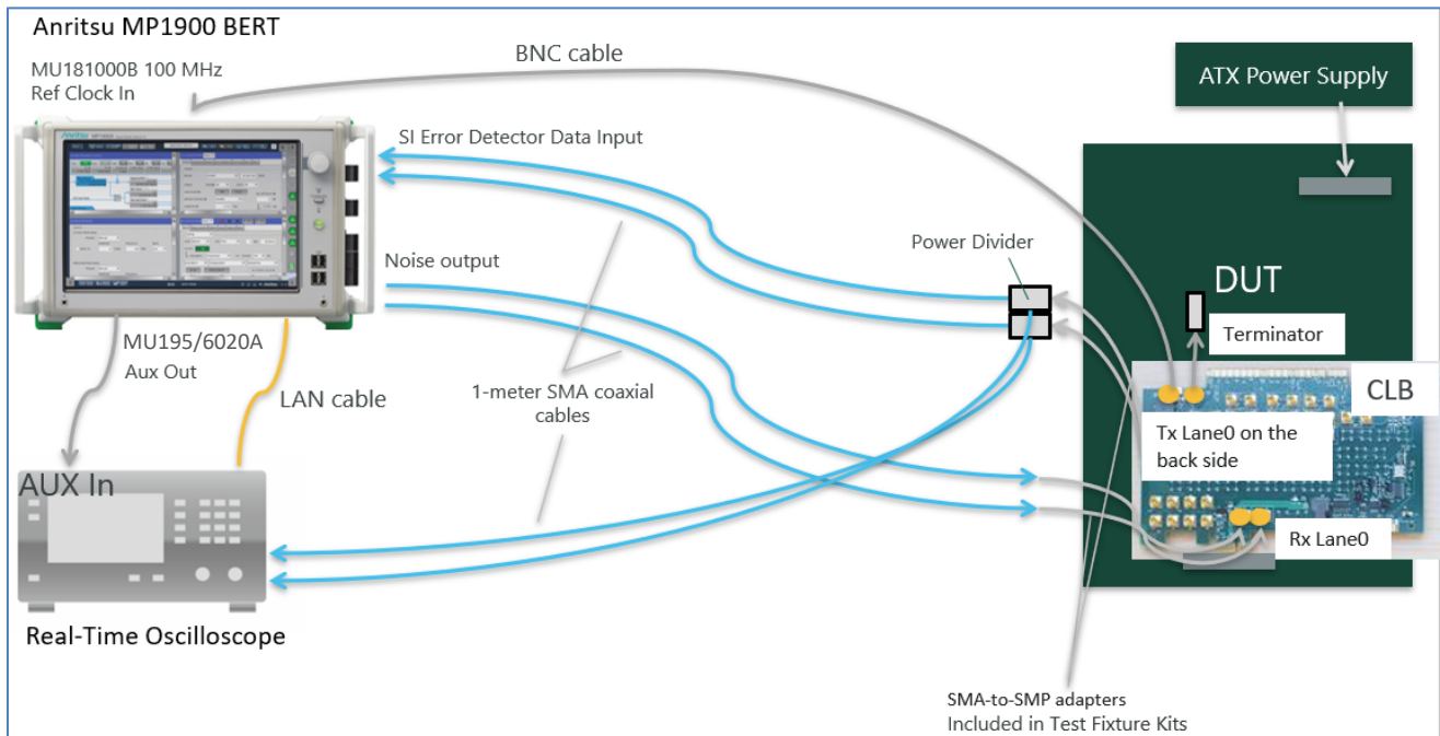
FIGURE 31. RECOMMENDED SETUP FOR DUT TX LINK EQ TESTING (PCIe GEN 3/4 SYSTEM BOARD)
