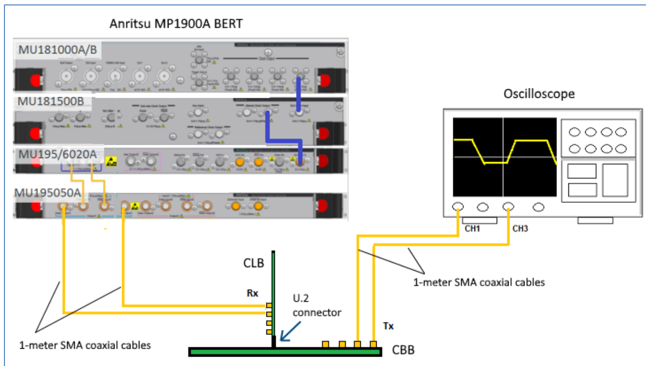
FIGURE 12. RECOMMENDED SETUP FOR U.2 TP2 LONG CHANNEL RX CALIBRATION (PCIe GEN 3 SYSTEM BOARD)
