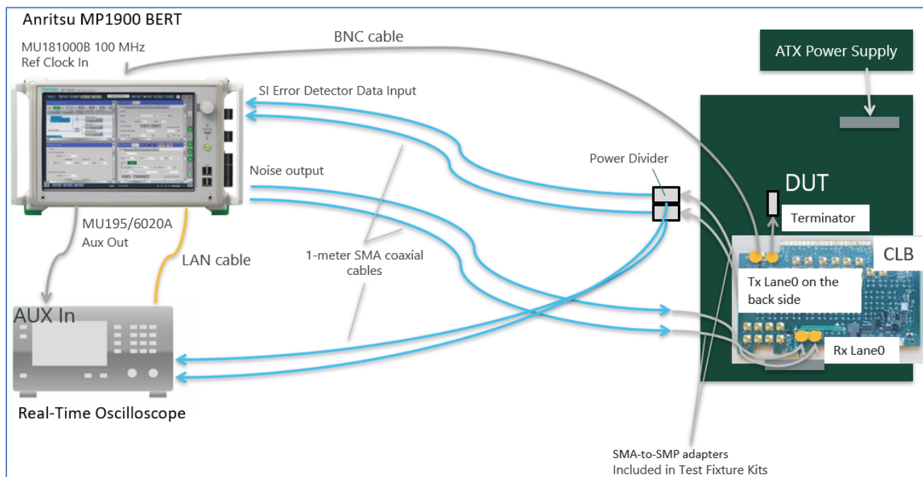
FIGURE 58. CONNECTION DIAGRAM FOR PCIe GEN 3/4 SYSTEM BOARD DUT TX LINK EQ RESPONSE TEST
