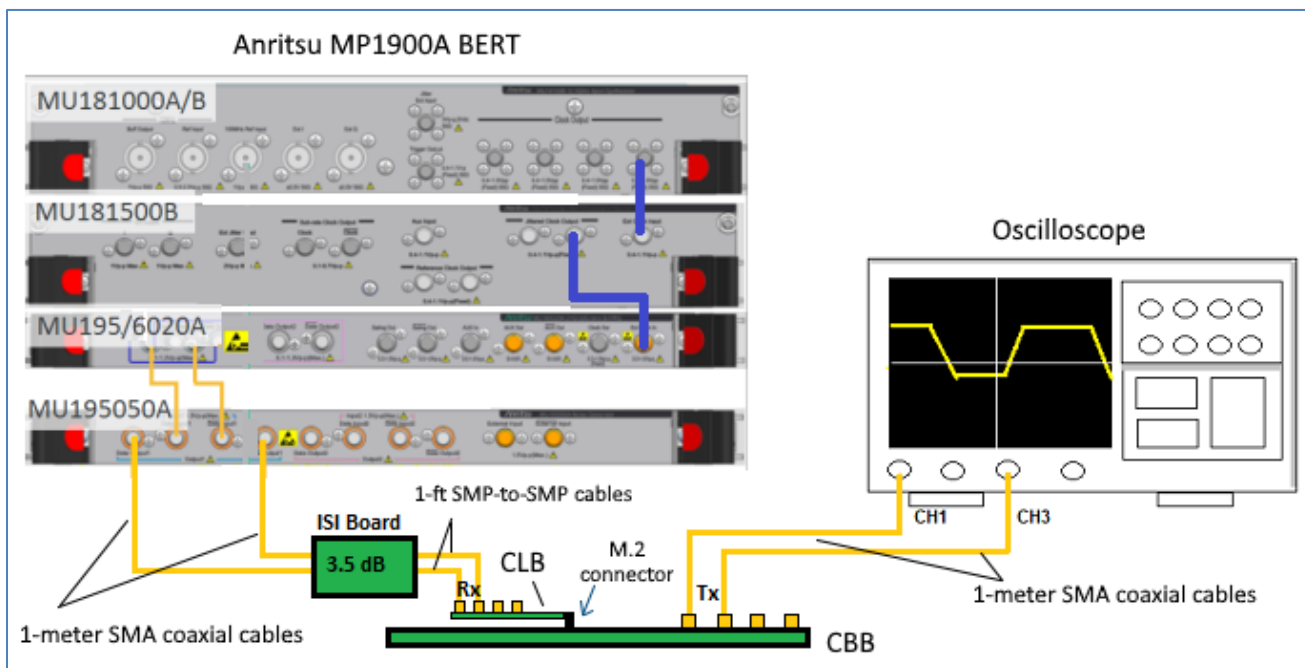
FIGURE 13. RECOMMENDED SETUP FOR M.2 TP2 LONG CHANNEL RX CALIBRATION (PCIe GEN 3 SYSTEM BOARD)
